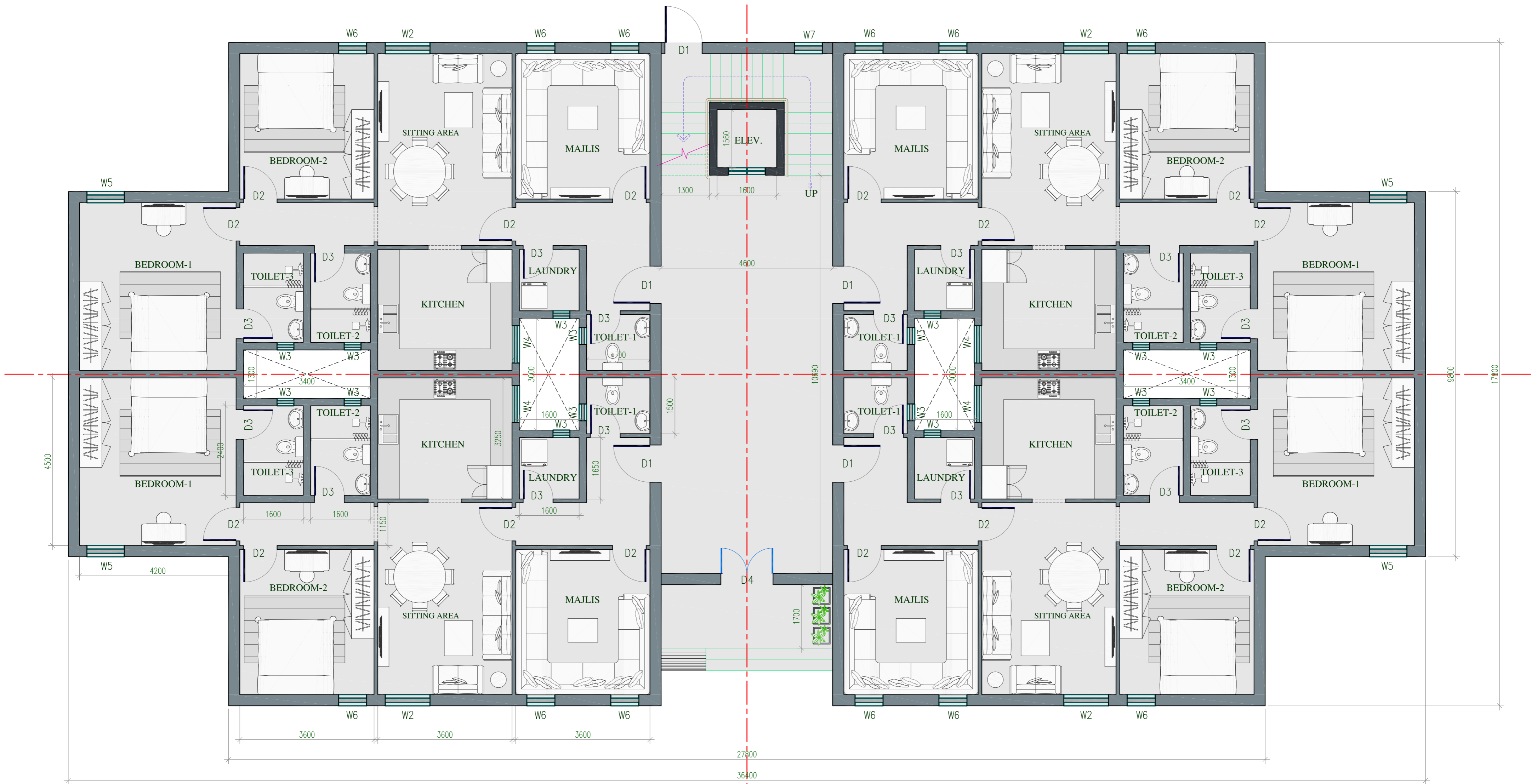
GROUND FLOOR 2 BED ROOM APARTMENT UNIT BUA 120.00Sqm. (One-Unit) Ref-06-0322
